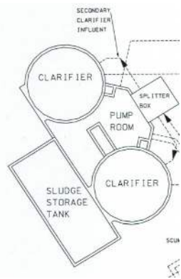
Figure 2. Diagram of WWTP
